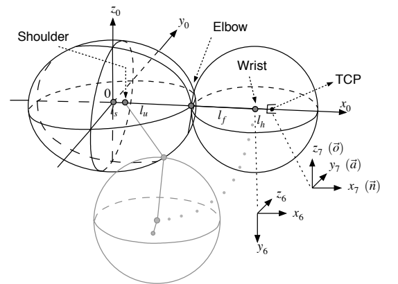
Fig. 3. Workspace of the upperarm and forearm
