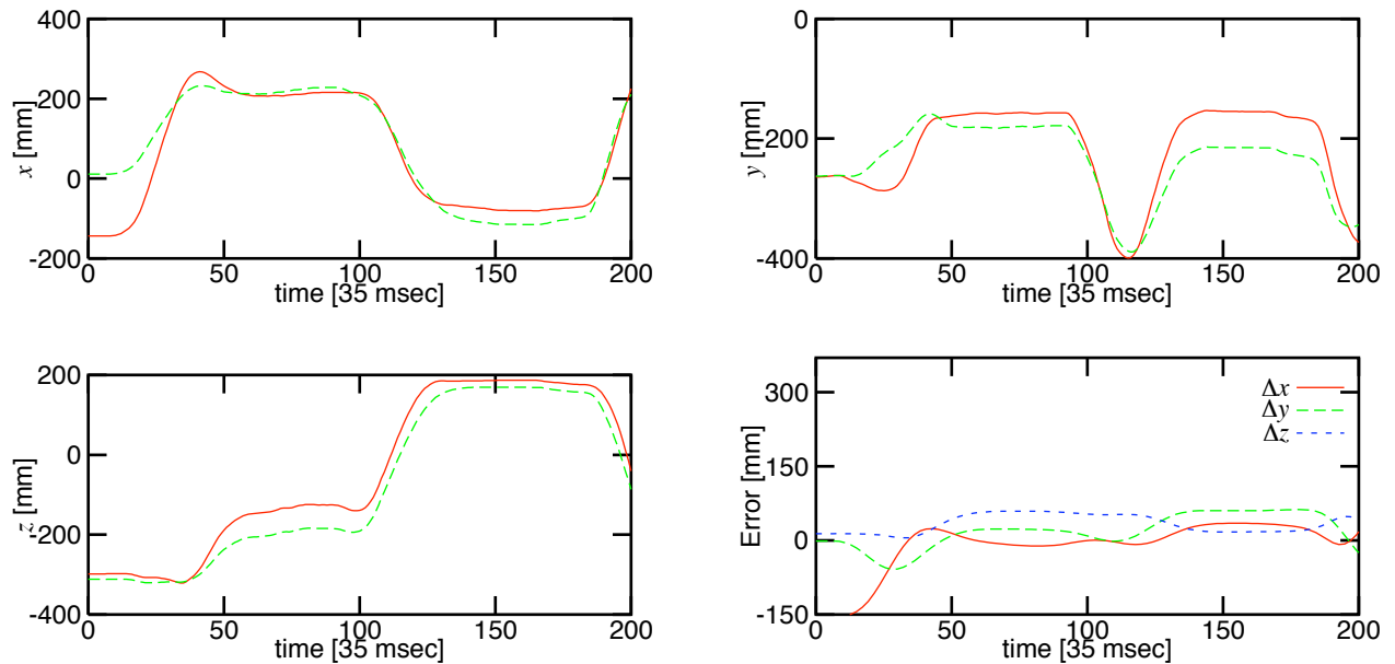
Fig. 8. Time history of the position trajectories.
