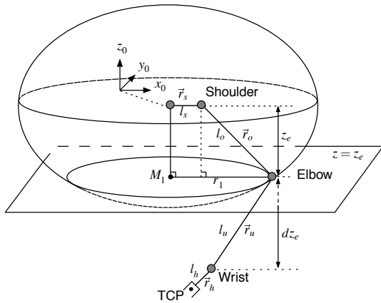
Fig. 4. The Ellipsoid and the plane z = z_e
