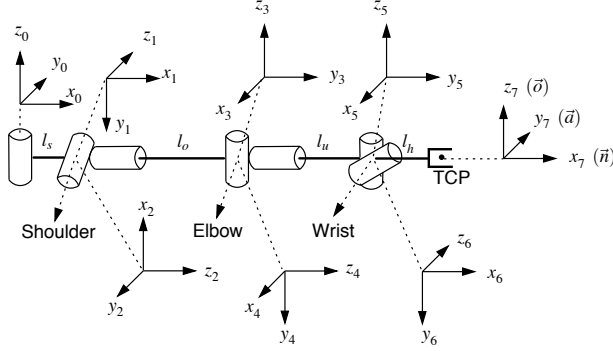
Fig. 2. Coordinate systems of the arm
