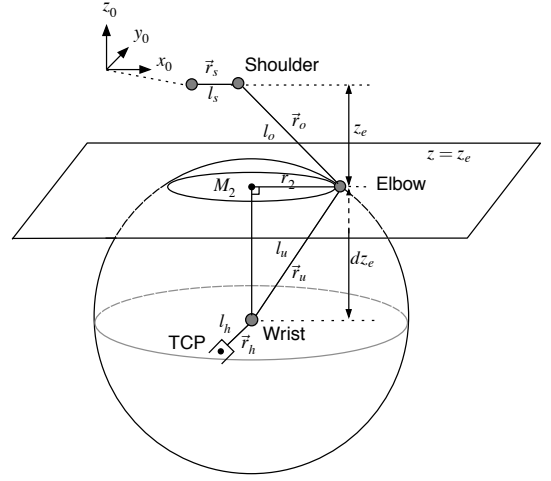
Fig. 5. The Sphere and the plane z = z_e
