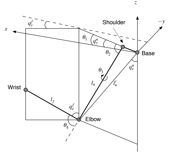
Fig. 7. Parameters for the humanoid arm posture.
